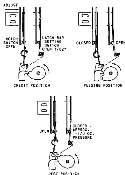
FIG. 7. MOTOR & LATCH BAR SETTING SWITCHES.
