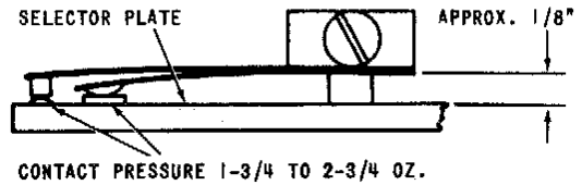
FIG. 10. CONTACT ARM.
