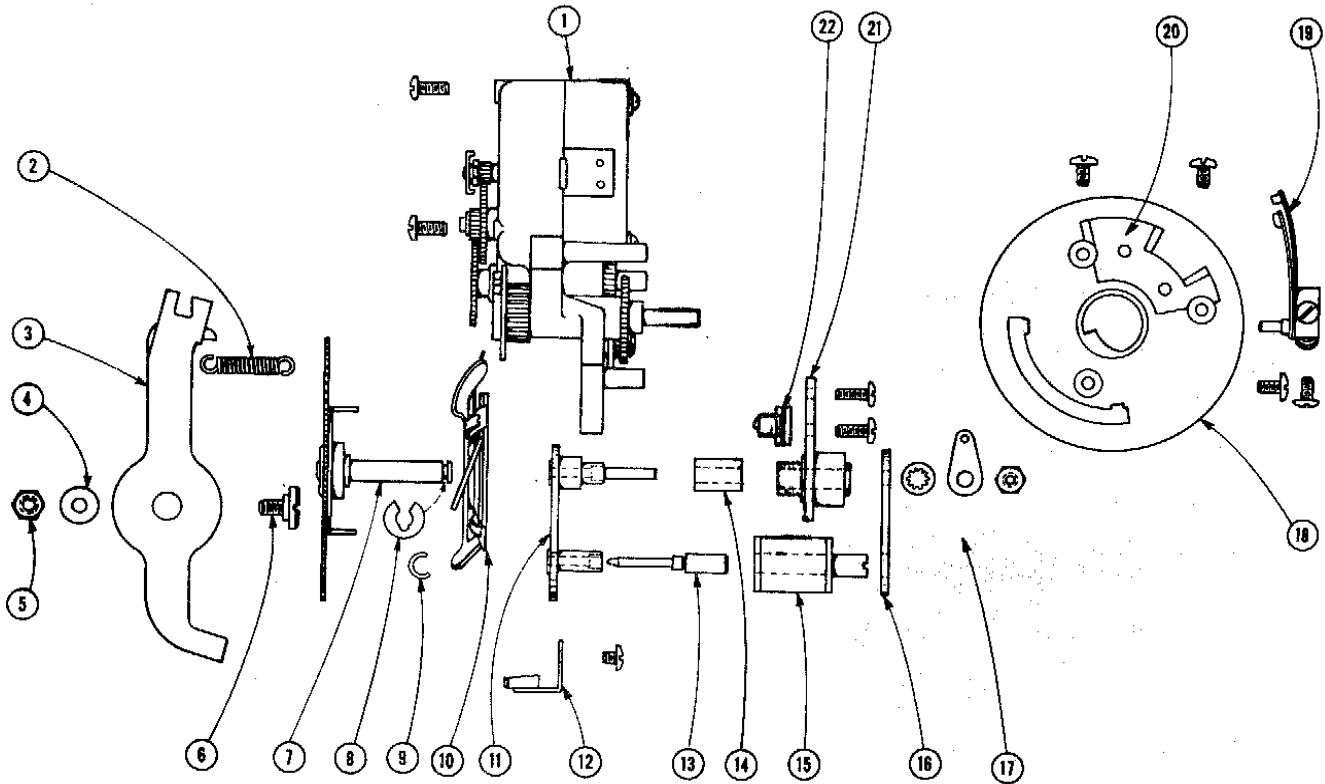
FIG. 22. MOTOR, CREDIT & CONTACT ASSEMBLY
