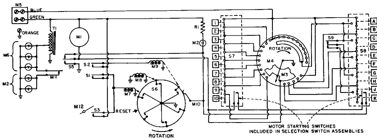
Figure 2. Schematic Diagram
