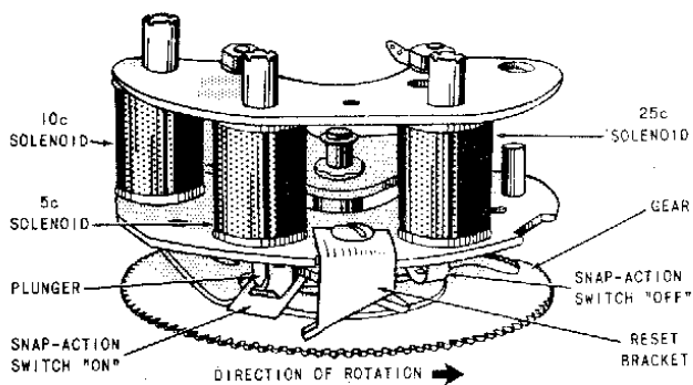
FIG. 5. CREDIT SOLENOID & SWITCH ASSEMBLY.
