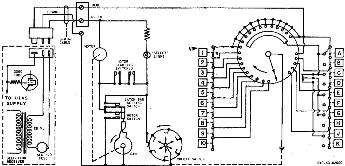
FIG. 2. SIMPLIFIED SCHEMATIC - 3W-1.
