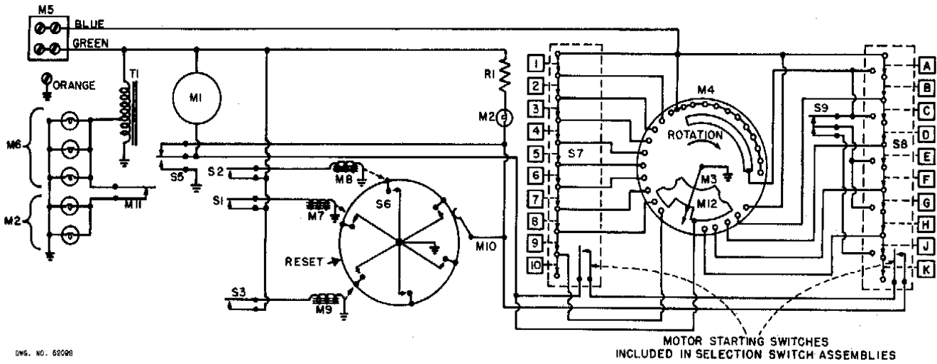
FIG. 17. SCHEMATIC DIAGRAM (ABOVE SERIAL NO. 16645)
