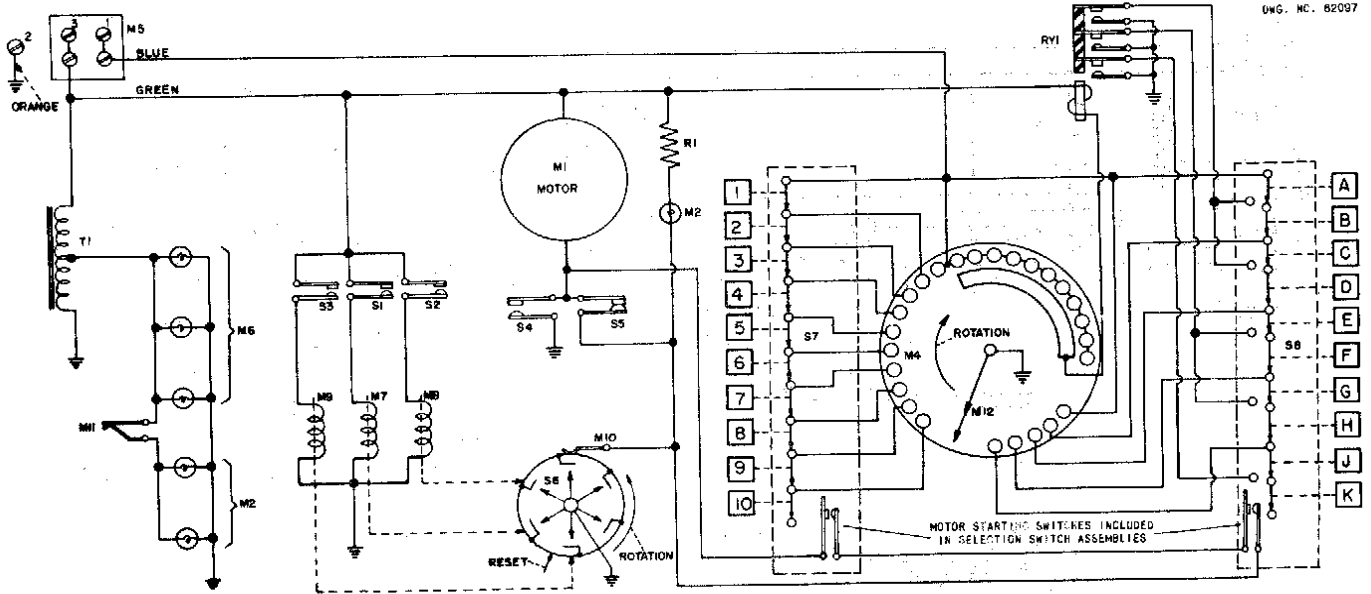
FIG. 15. SCHEMATIC DIAGRAM (BELOW SERIAL NO 2303)
