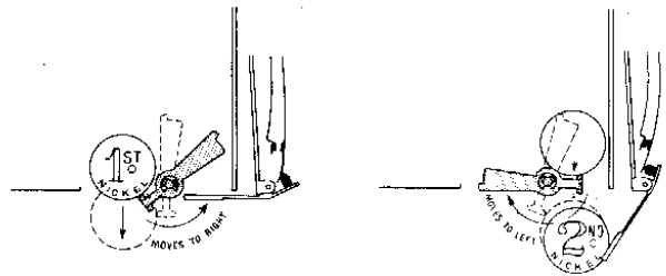
Figure 1. Nickel Diverter
