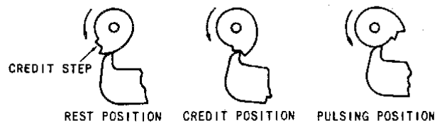
FIG. 3. CAM POSITIONS.
