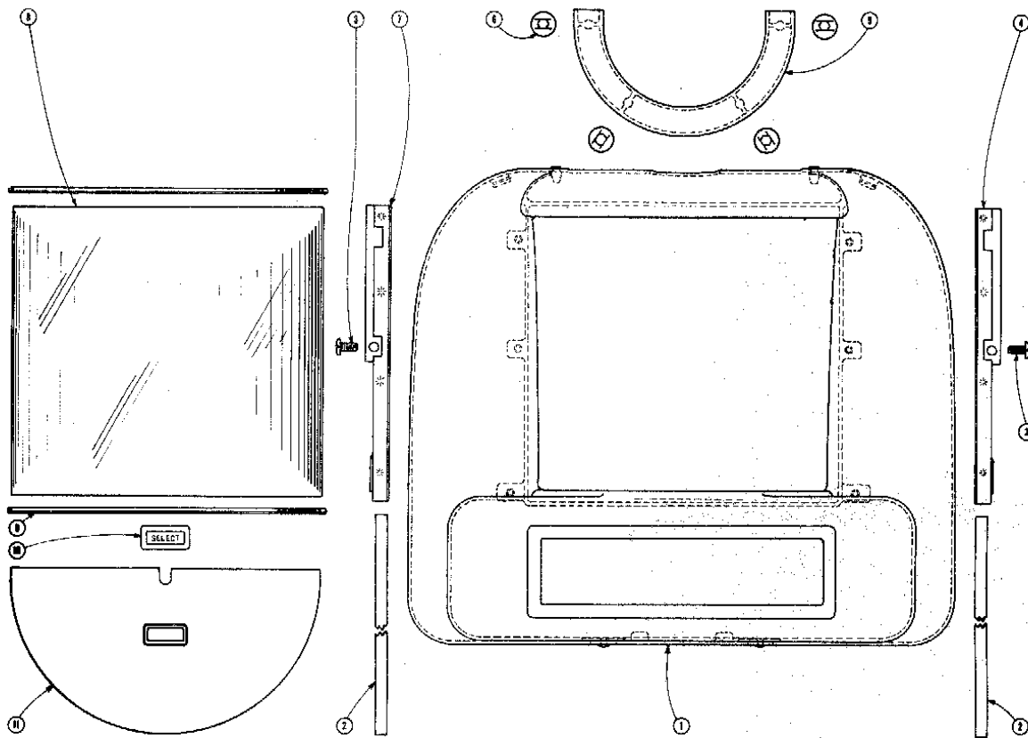
FIG. 18. HOUSING ASSEMBLY
