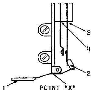
FIG. 6A. COIN SWITCH ADJUSTMENTS.
