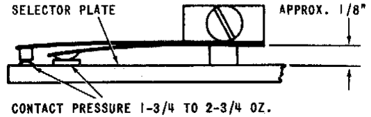
FIG. 10. CONTACT ARM.
