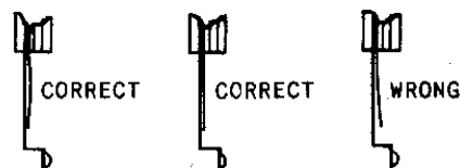
FIG. 6B. COIN SWITCH ADJUSTMENTS.
