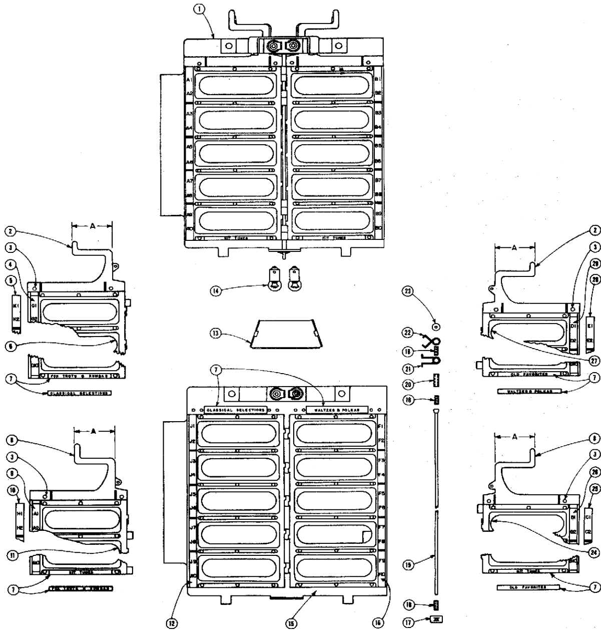
FIG. 20. PROGRAM HOLDER ASSEMBLY
