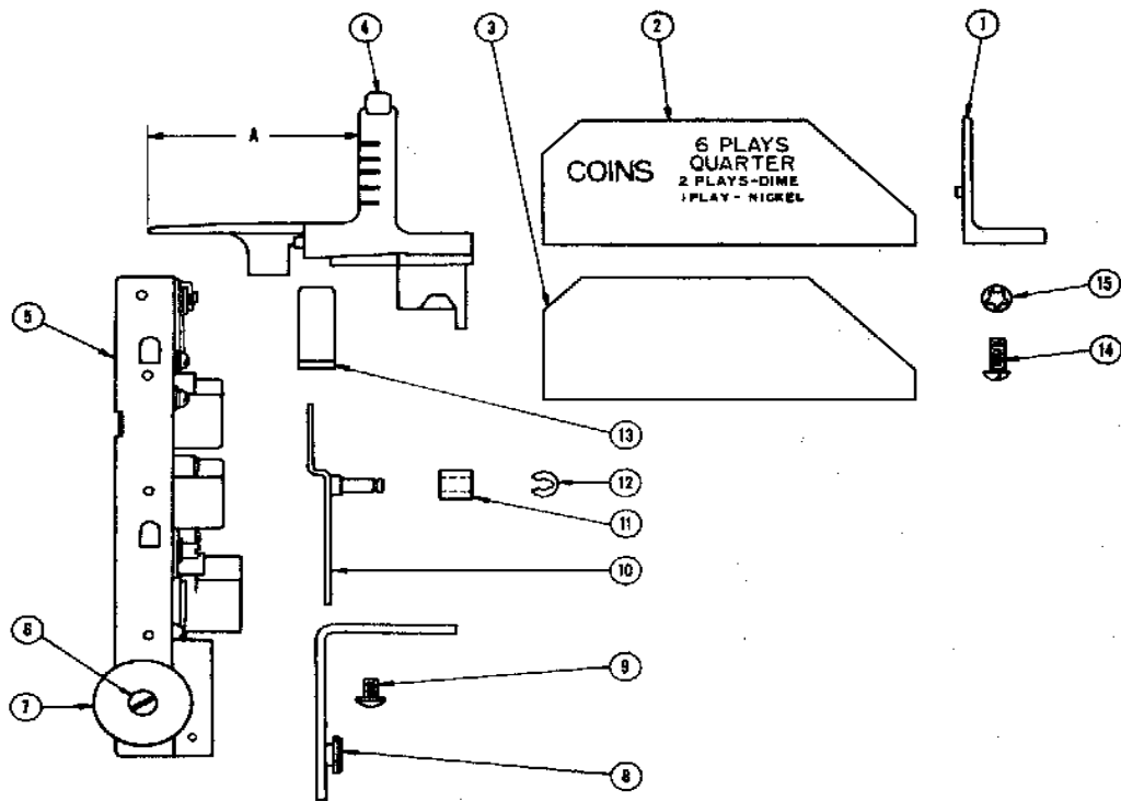
FIG. 19. COIN EQUIPMENT
