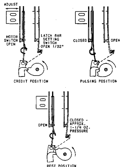
FIG. 7. MOTOR & LATCH BAR SETTING SWITCHES.
