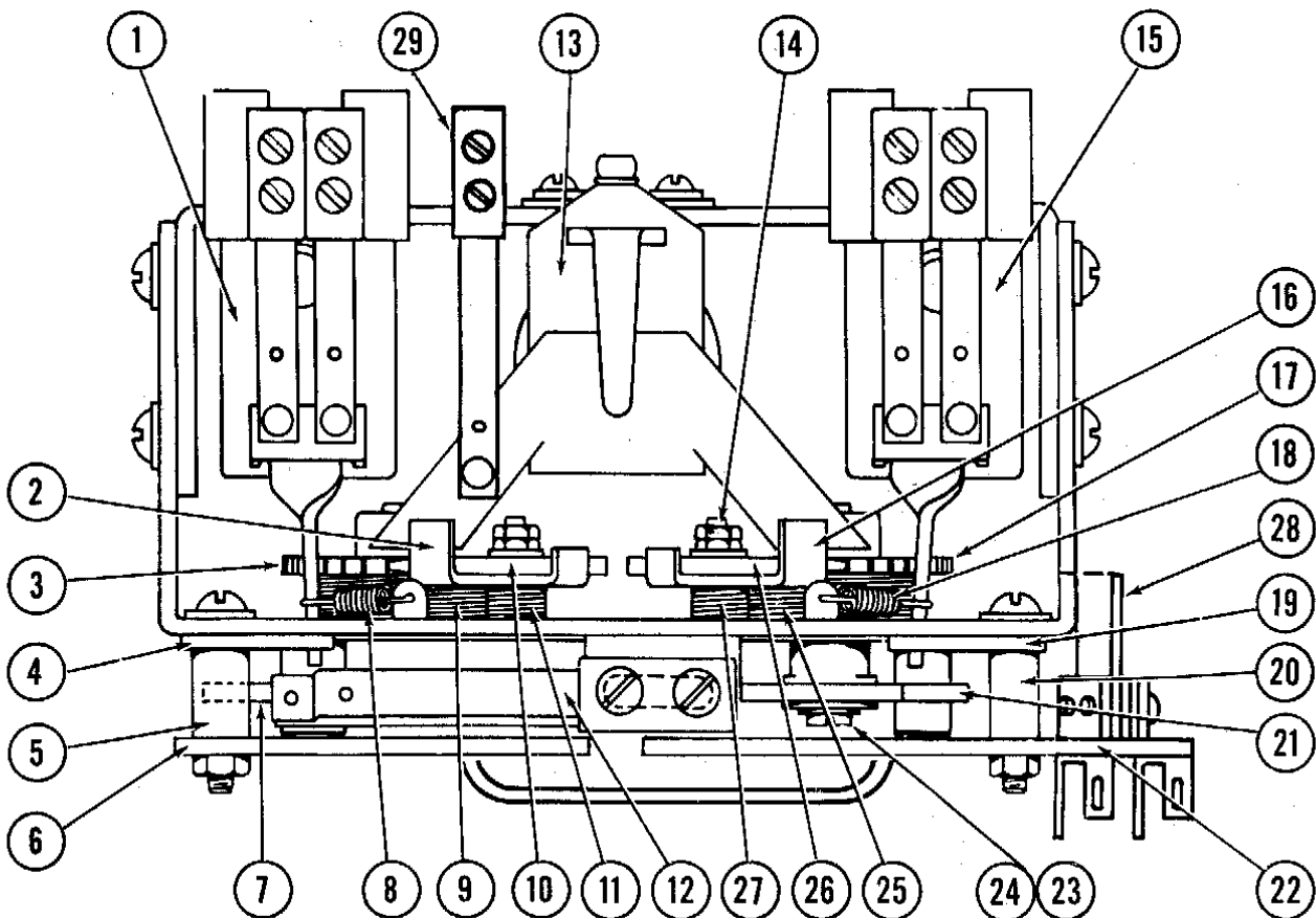
Figure 21. No. 303510 Assembly
