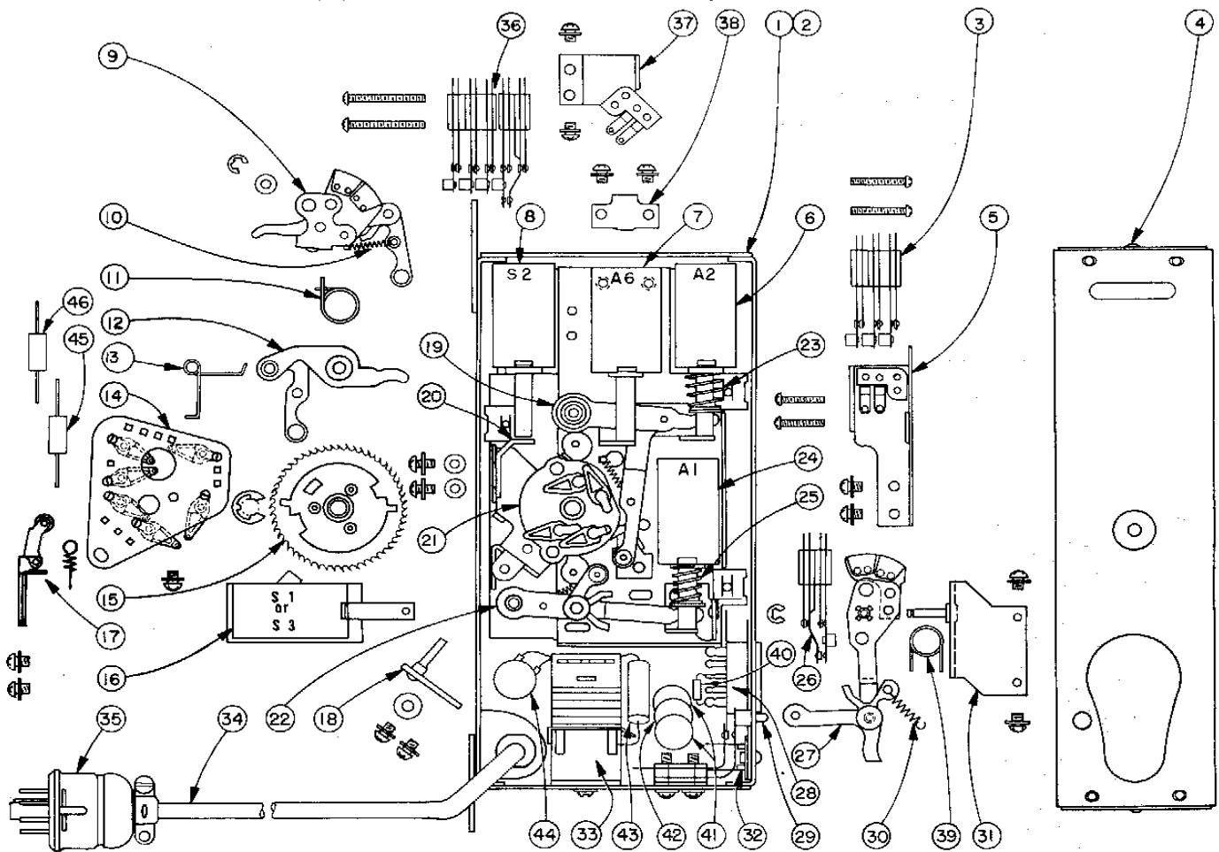
Figure 22. Dual Credit Unit Assemblies
