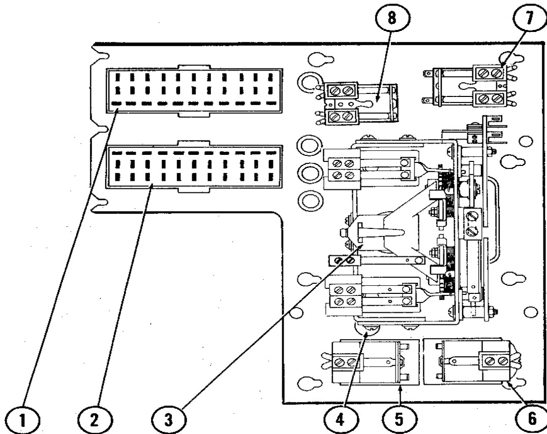
Figure 20. No. 303520 Step Switch & Relay Assembly
