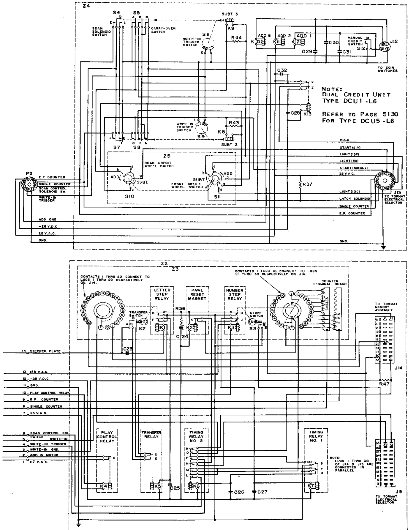
Figure 18. - Schematic Diagram
