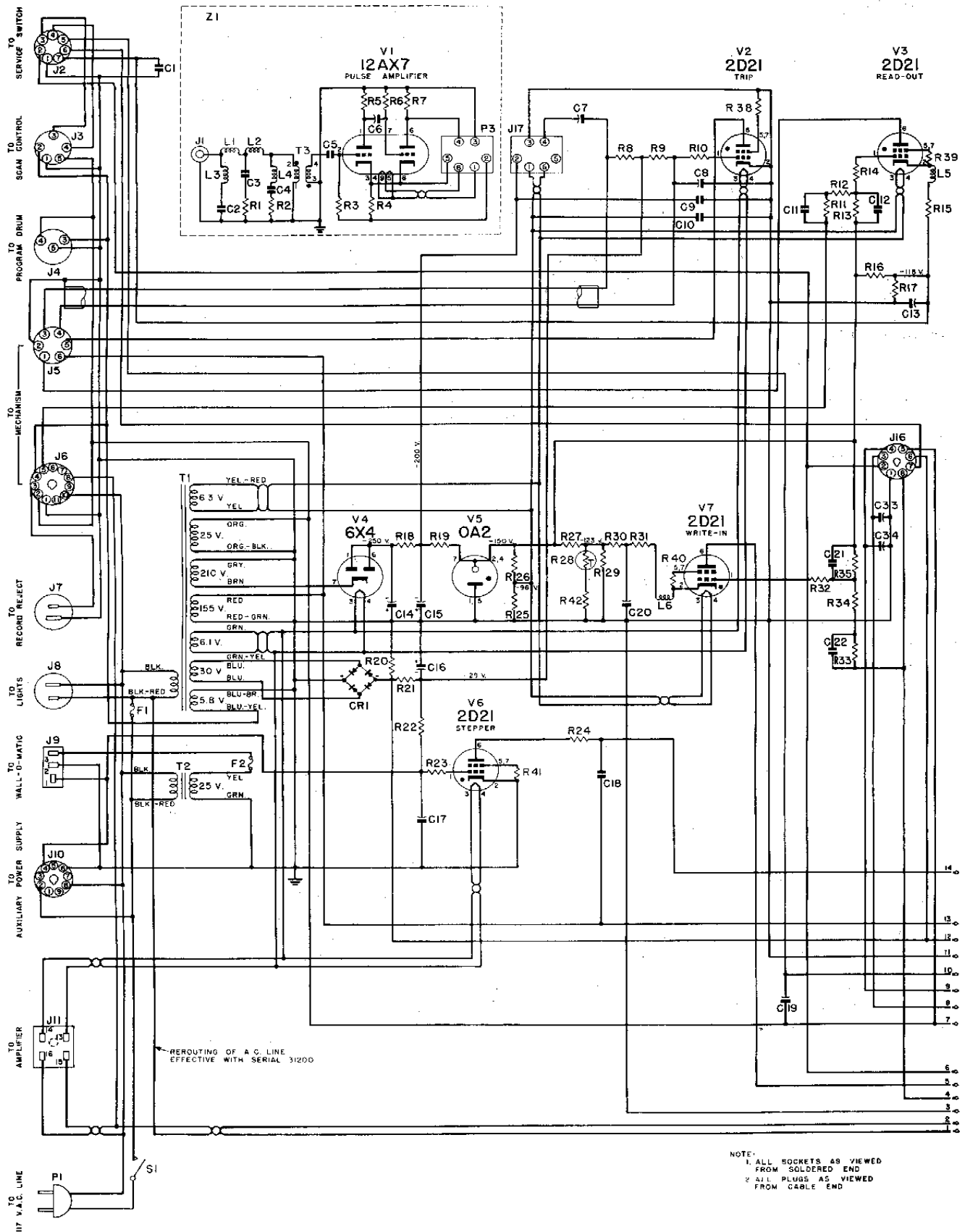
Figure 17. - Schematic Diagram
