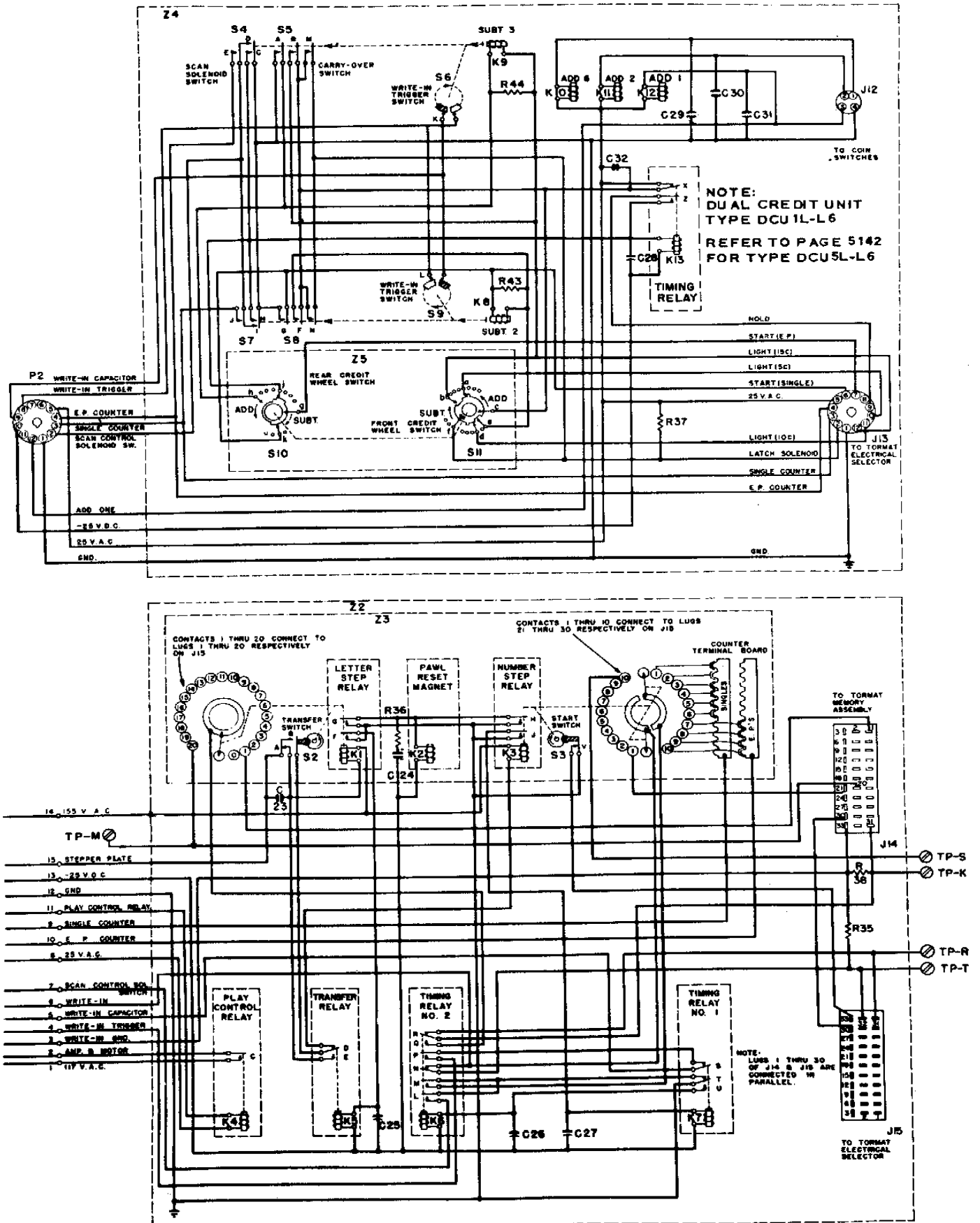
Schematic Diagram
