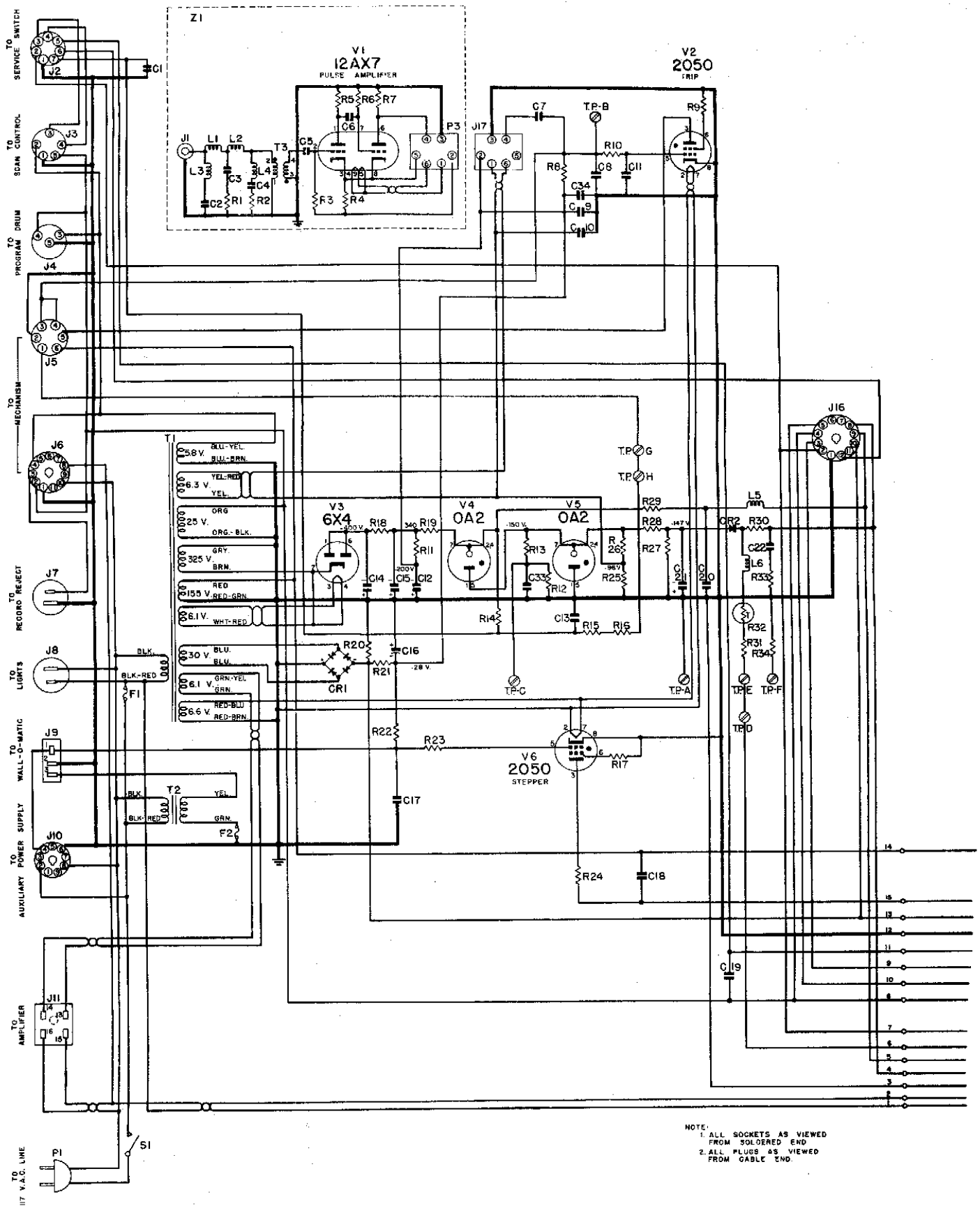
Schematic Diagram
